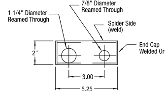
TOP RECEIVER FRAME
